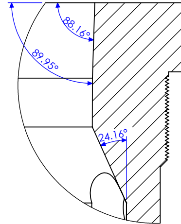
DETAIL O SCALE 1 : 1
