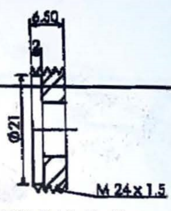
SECTION C-C
