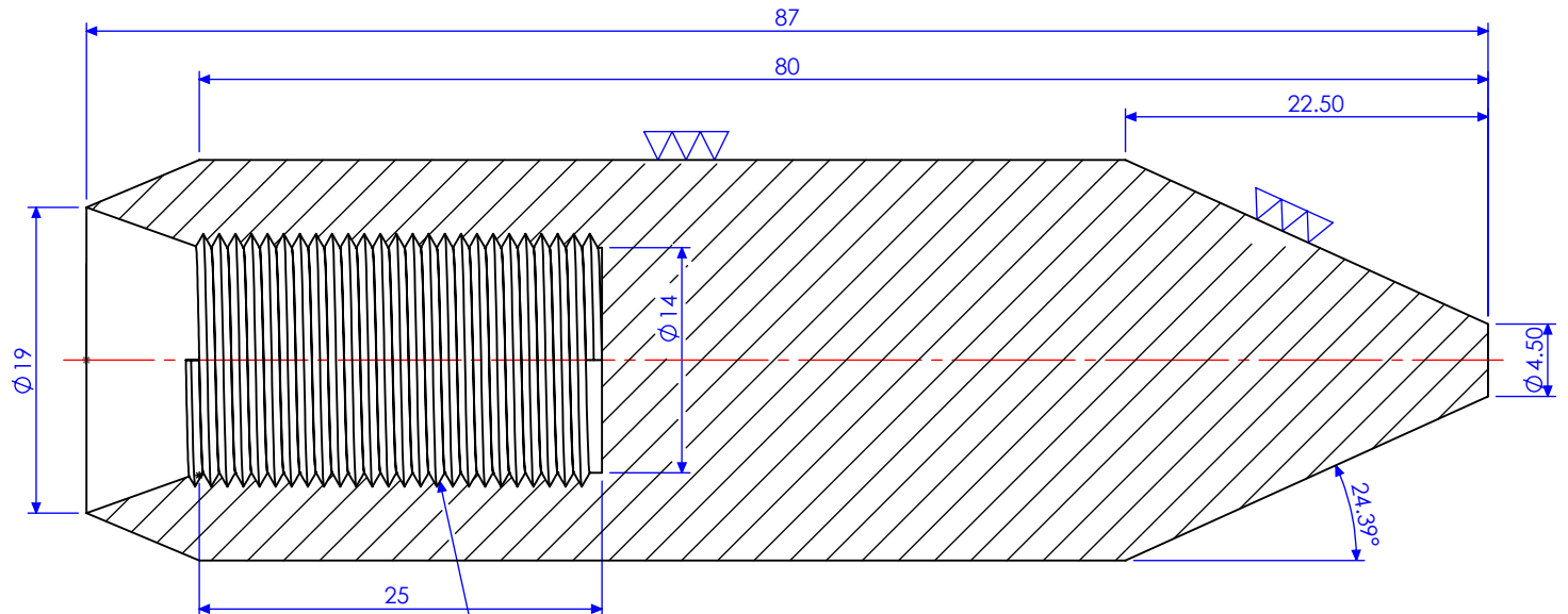
SECTION L-L
